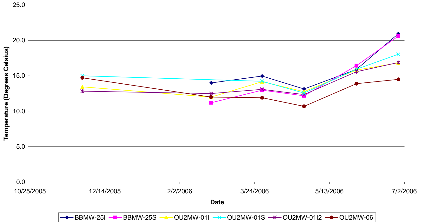
Figure C5 Groundwater Temperature Data Bay Shore/Brightwaters Former MGP Site Operable Unit 2 (OU-2) Bay Shore, New York
