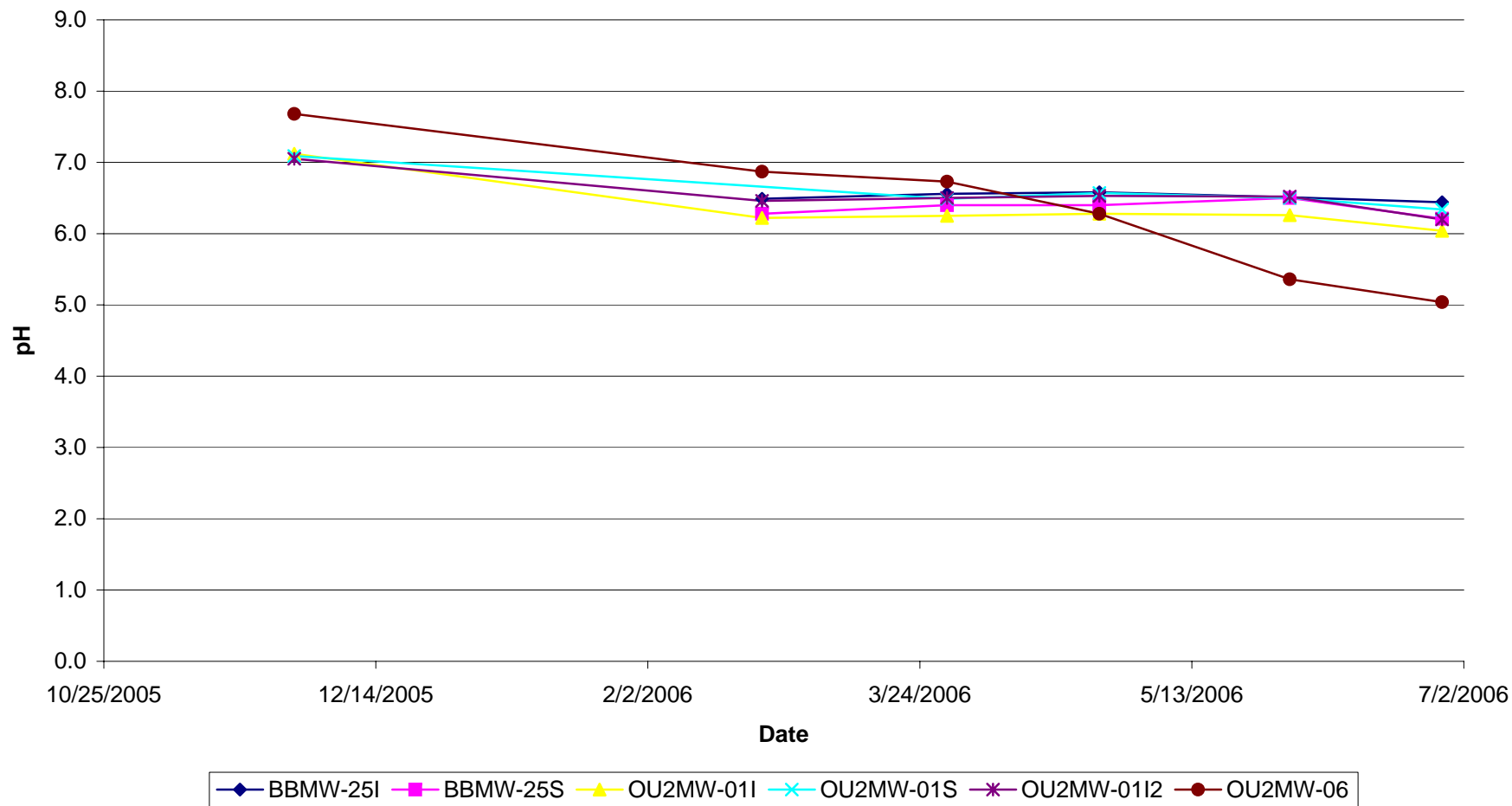
Figure C3 Groundwater pH Data Bay Shore/Brightwaters Former MGP Site Operable Unit 2 (OU-2) Bay Shore, New York
