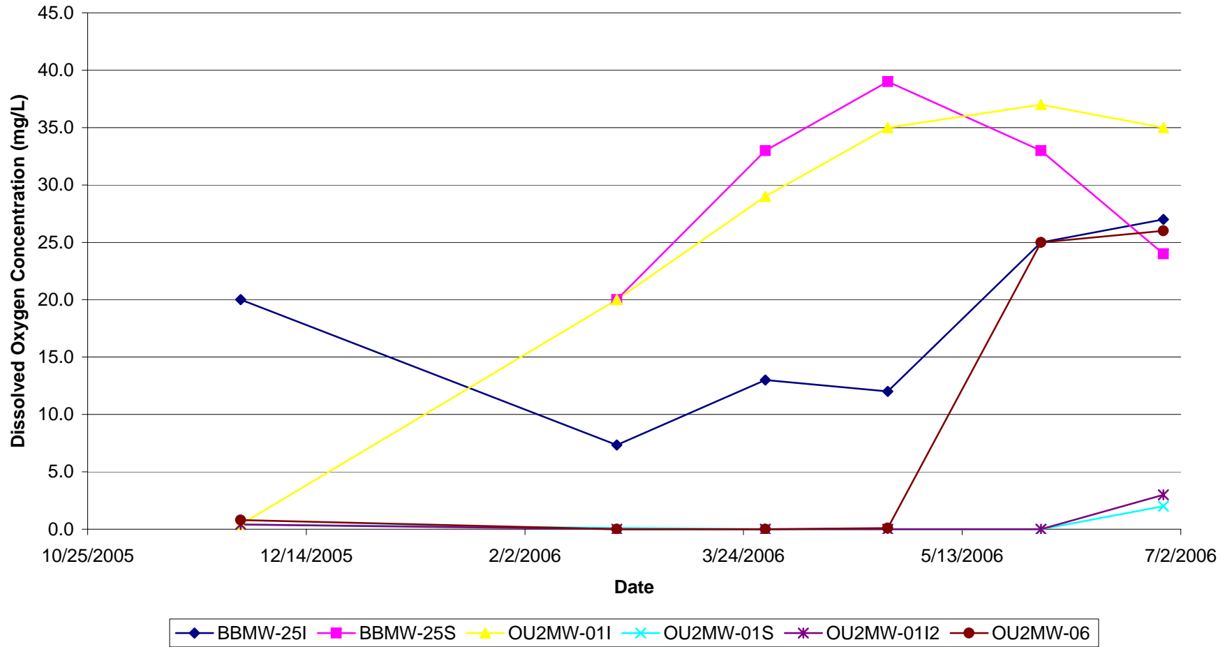
Figure C1 Groundwater Dissolved Oxygen (DO) Concentration Data Bay Shore/Brightwaters Former MGP Site Operable Unit 2 (OU-2) Bay Shore, New York
