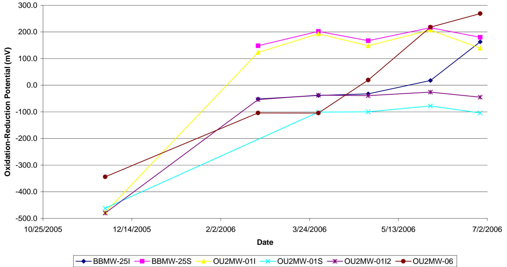
Figure C4 Groundwater Oxidation-Reduction Potential (ORP) Data Bay Shore/Brightwaters Former MGP Site Operable Unit 2 (OU-2) Bay Shore, New York
