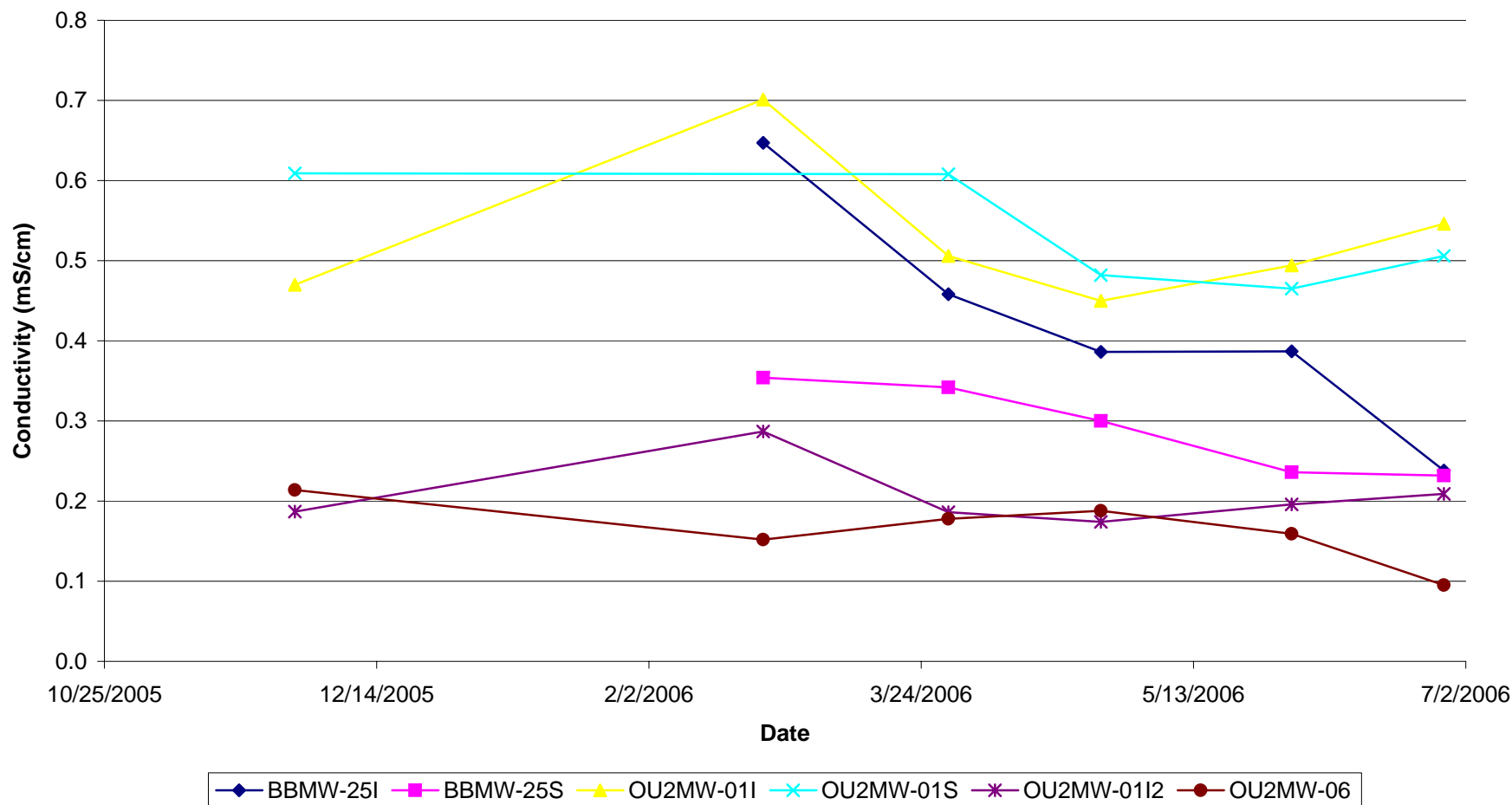
Figure C2 Groundwater Conductivity Data Bay Shore/Brightwaters Former MGP Site Operable Unit 2 (OU-2) Bay Shore, New York
